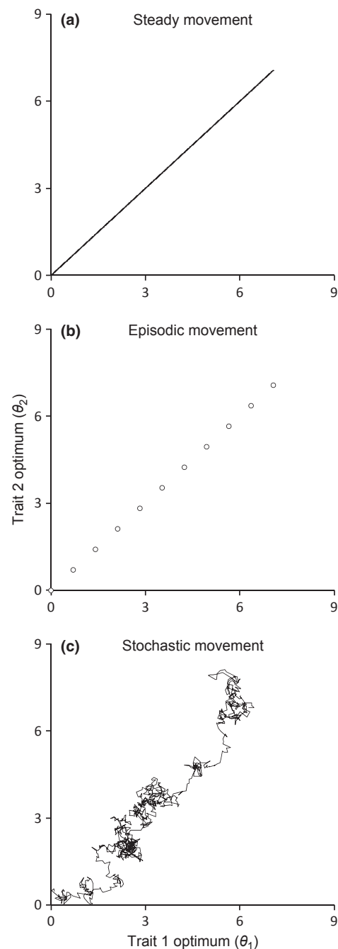
Fig. 1 Schematic portrayals of the three modes of peak movement used in the simulations. In all of these figures, the peak starts at (or near) the origin and moves up and to the right. In (a), the peak moves every generation in a constant direction at a constant rate. In (b) and (c), the average rate and direction are as in (a). In (b), the peak remains stationary for many generations and then jumps to the new position. In the case shown, the jumps occur every 100 generations. In (c), the peak moves every generation, but peak movement also includes an element of stochasticity each generation. In this case, the stochasticity variance parameter ( \sigma_\theta^2 ) is 0.01.
